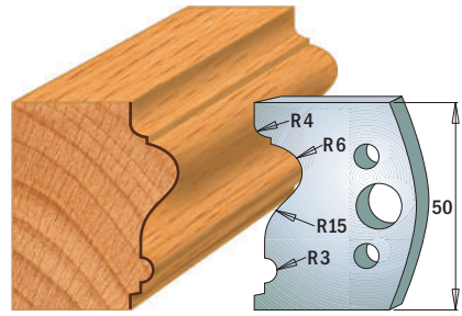
Pair of knives 690.512
